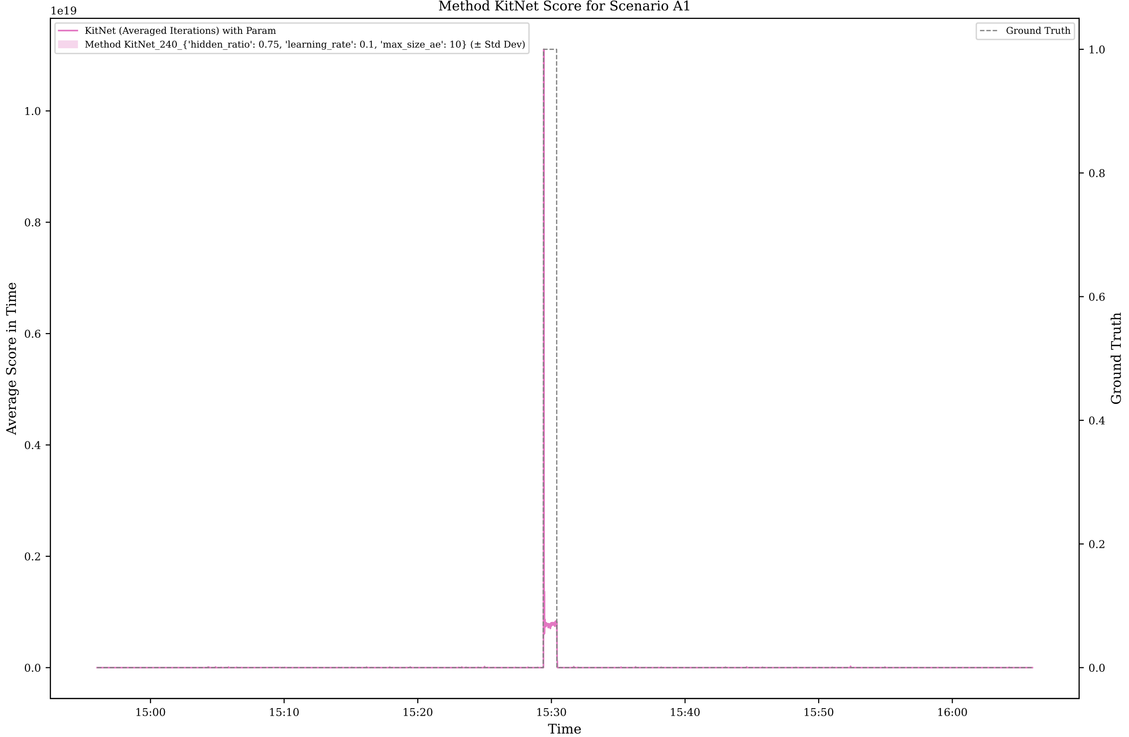
Method KitNet Score for Scenario A1
